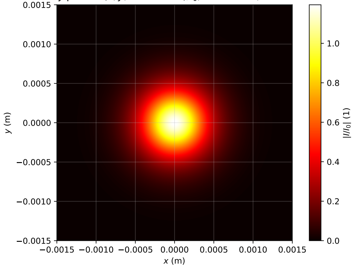
Intensity profile I(x, y, z = 0.955m)/I_0 , P_{in}=0.7P_{cr} , artificial time
